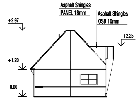
CROSS SECTION 1-1
